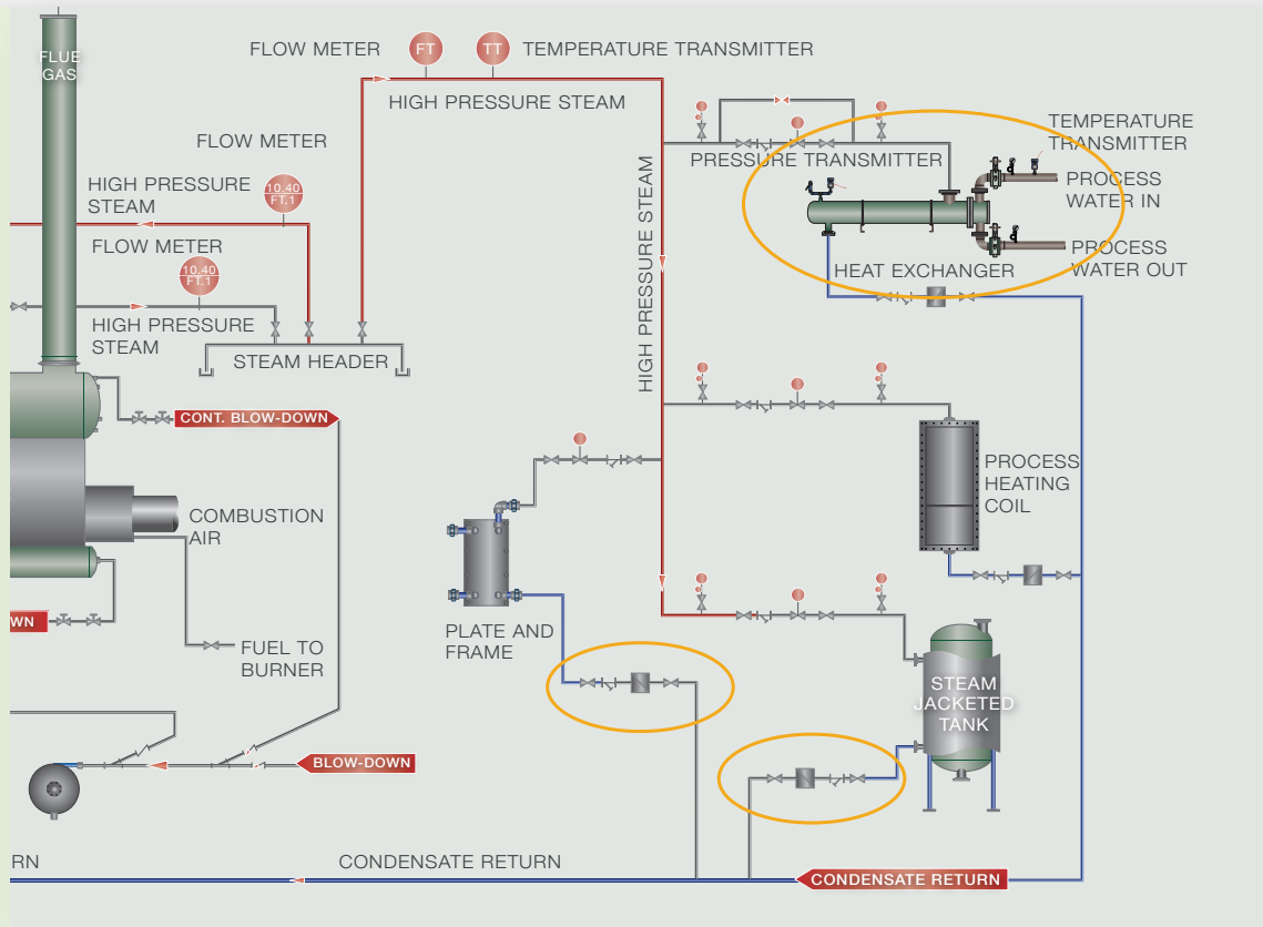
Figure 7: Steam End Users Thermal Losses
