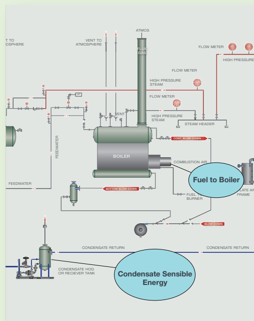
Figure 2: Energy in and Returned
