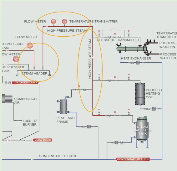
Figure 5: Steam Distribution Losses
