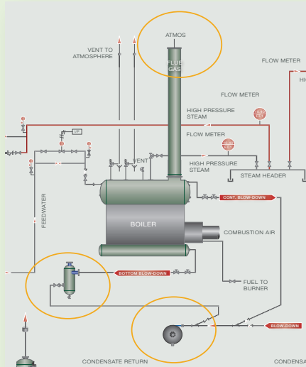
Figure 3: Losses in the Steam Generation Area
