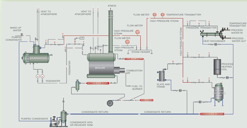
Figure 1: Total Steam System
