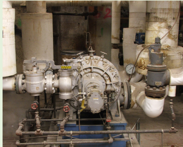
Figure 4: Small Steam Turbine Installation
